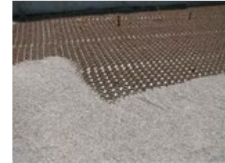
GRAVELPAVE2 DURING INSTALLATION
