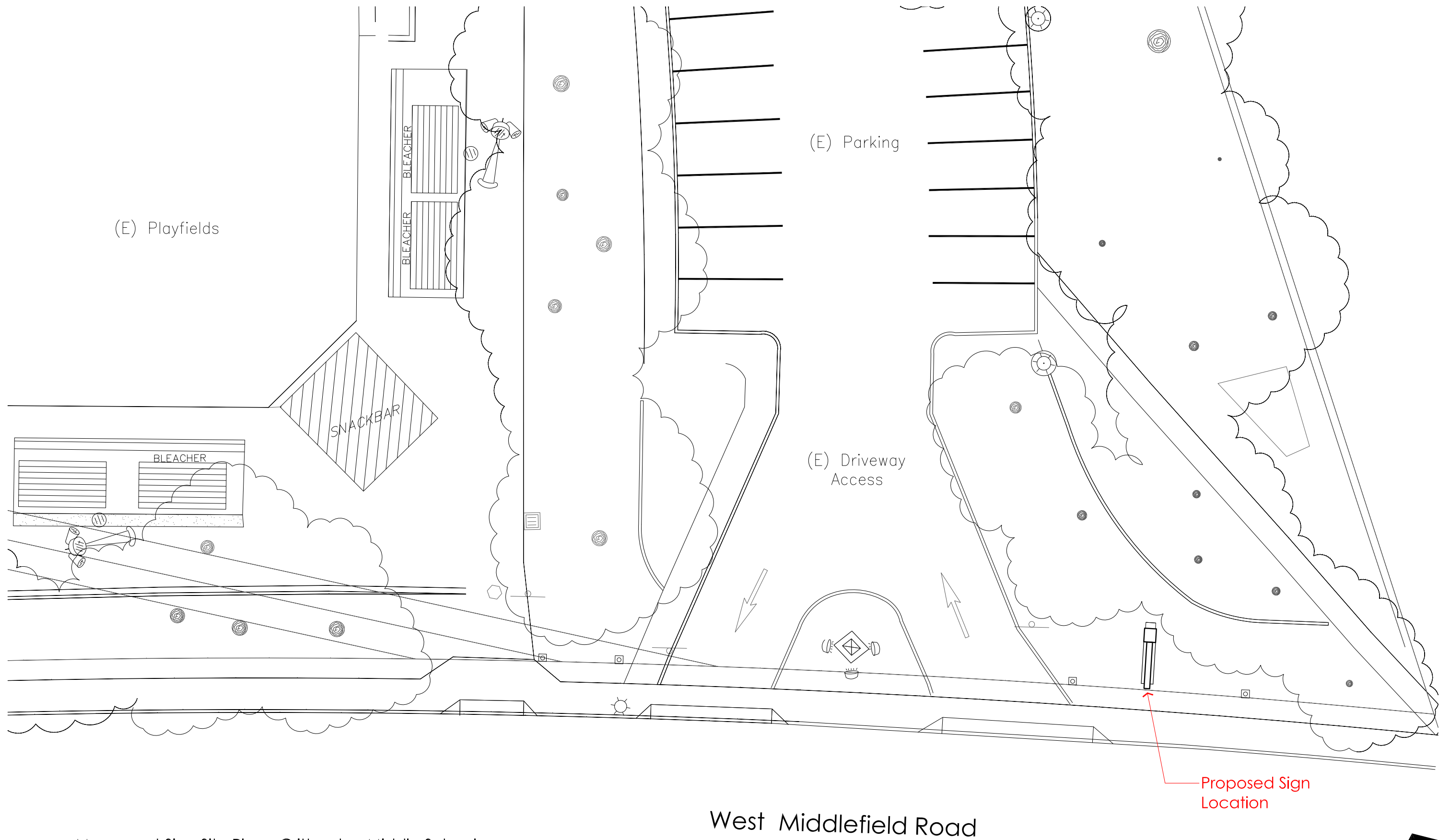
1 Monument Sign Site Plan - Crittenden Middle School
